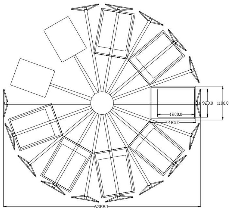
PRISM I 18s 16c (91 x 110 cm print area configuration)
