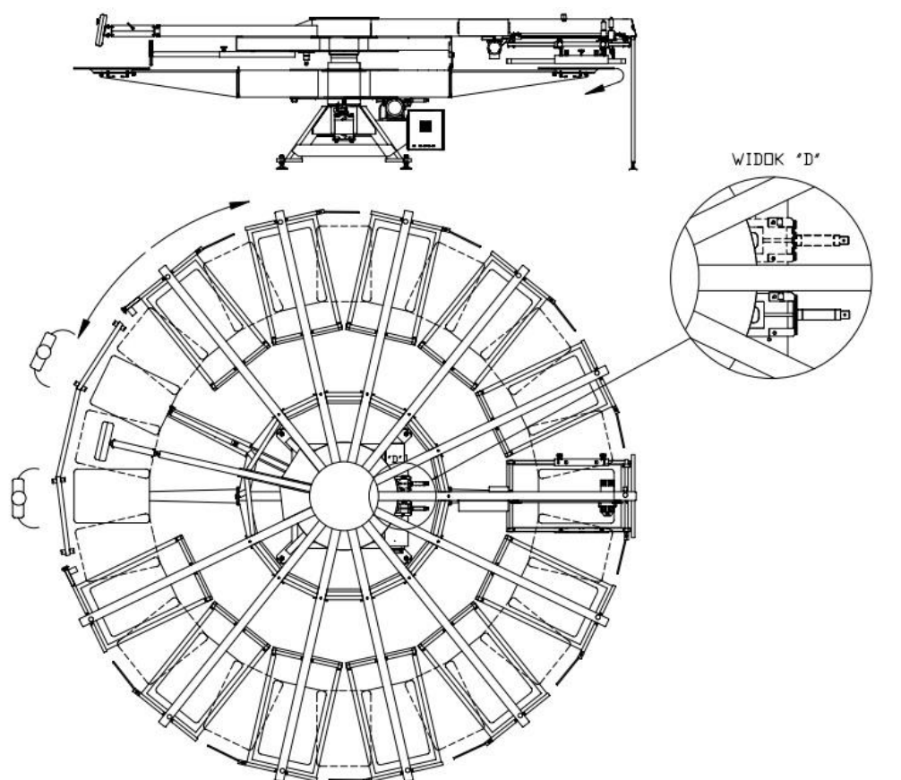
PRISM I 14s 12c side screen holders version
