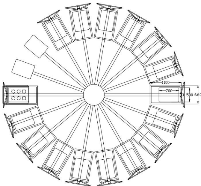
PRISM I 18s 16c (50 x 70 cm print area configuration)
