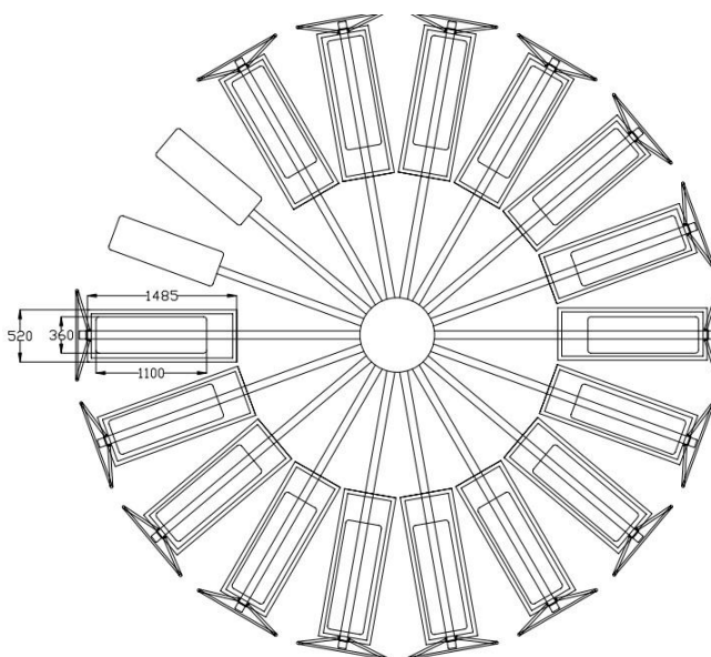
PRISM I 18s 16c (36 x 110 cm print area configuration)
