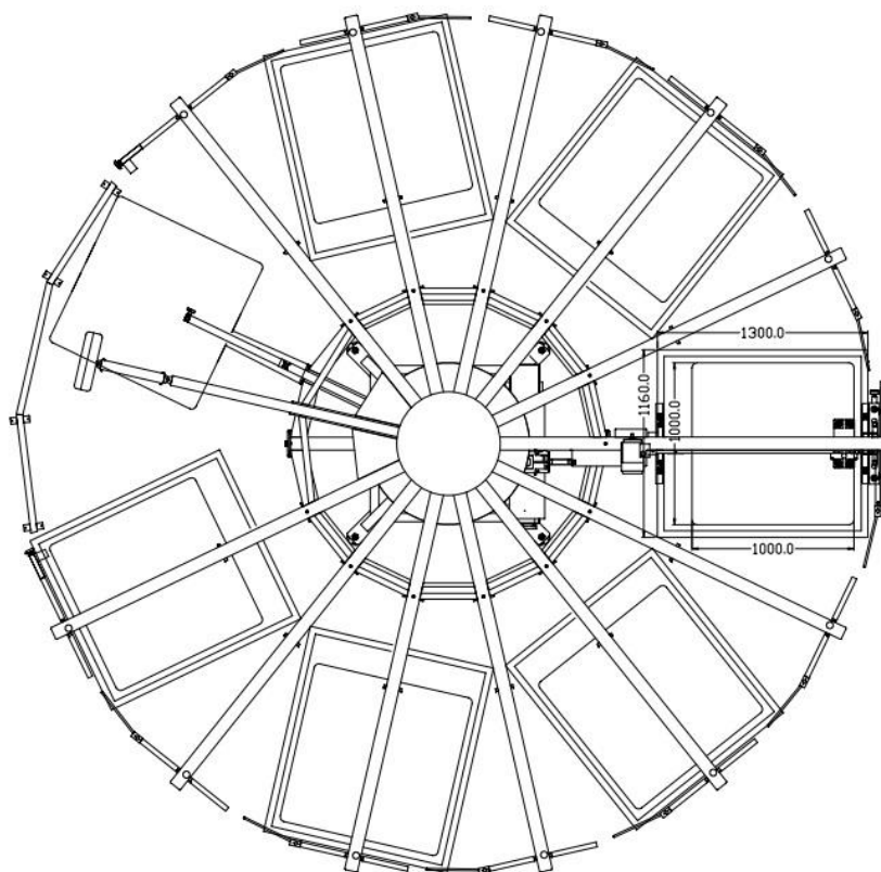
PRISM I 14s 12c 100 x 90 cm print area configuration (Every second color)
